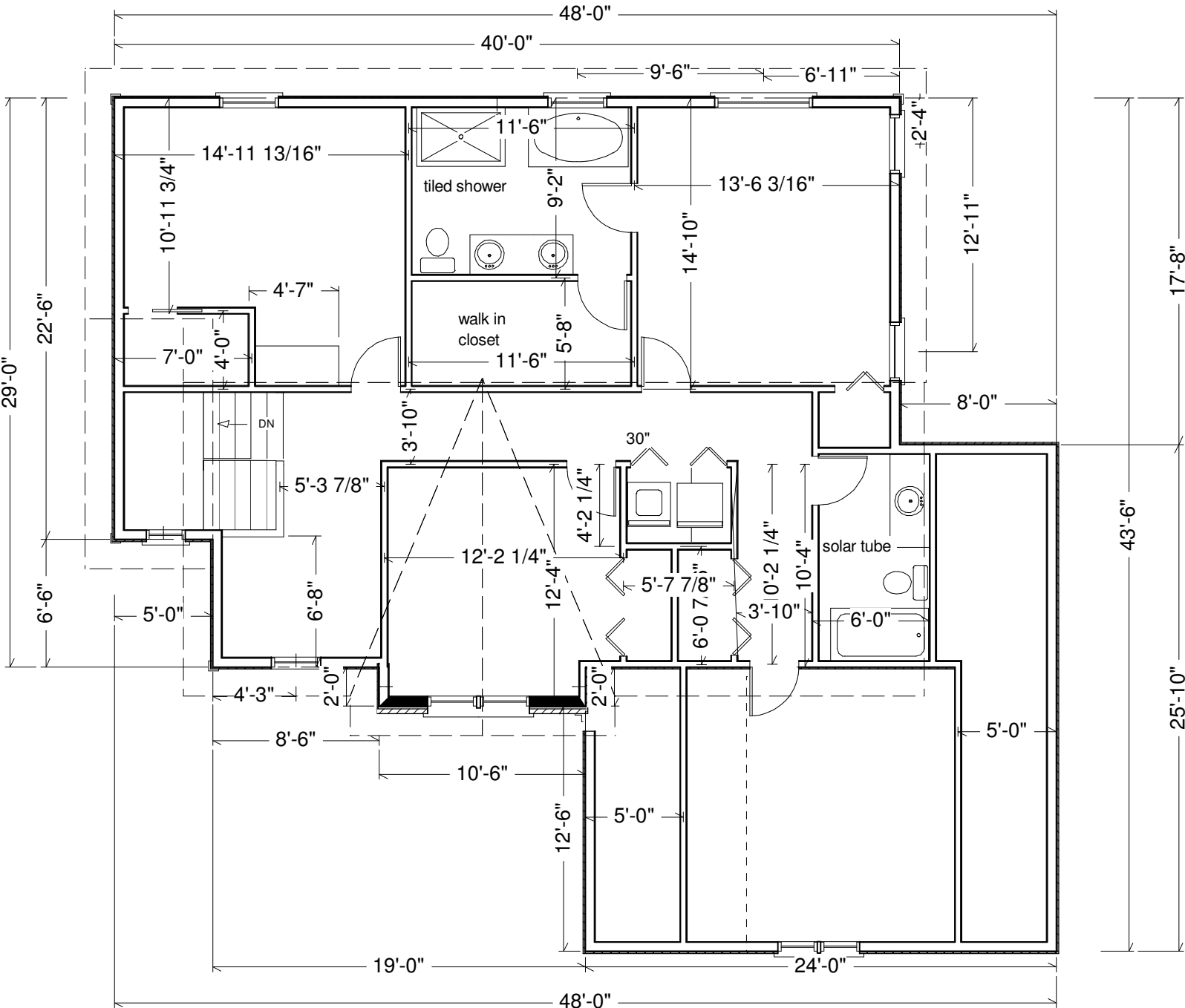
LIVING AREA 1316 sq ft
